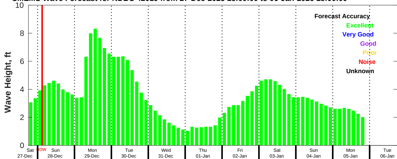
CMEMS Wave Forecast for NDBC 42019 from 27-Dec-2025 18:00:00 to 06-Jan-2026 18:00:00
