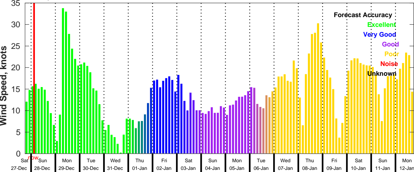
GFS Wind Speed Forecast for NDBC 42019 from 27-Dec-2025 18:00:00 to 12-Jan-2026 18:00:00
