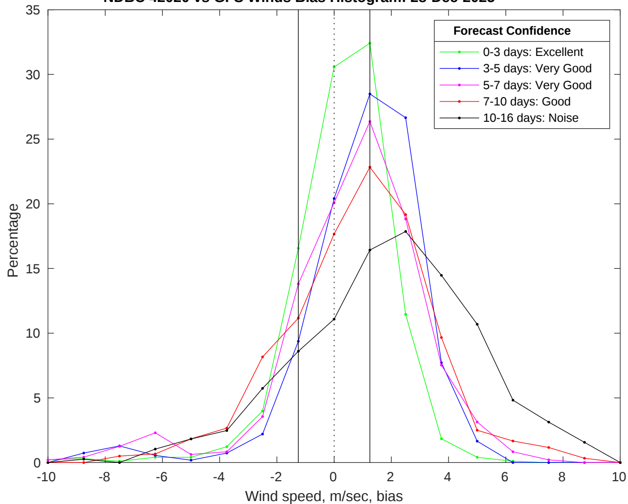
NDBC 42020 vs GFS Winds Bias Histogram: 28-Dec-2025
