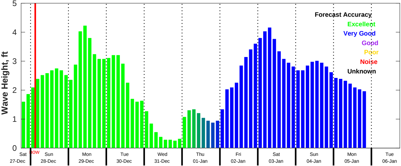
CMEMS Wave Forecast for NDBC 42035 from 27-Dec-2025 18:00:00 to 06-Jan-2026 18:00:00
