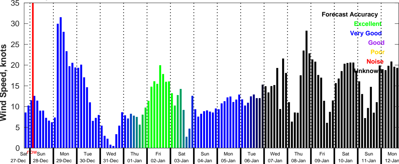
GFS Wind Speed Forecast for NDBC 42035 from 27-Dec-2025 18:00:00 to 12-Jan-2026 18:00:00
