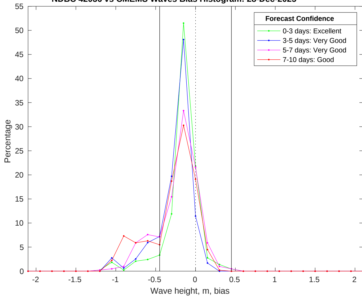
NDBC 42036 vs CMEMS Waves Bias Histogram: 28-Dec-2025
