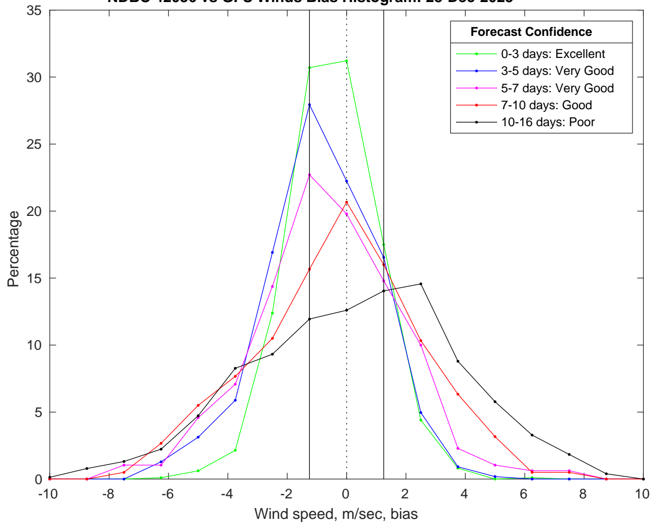
NDBC 42036 vs GFS Winds Bias Histogram: 28-Dec-2025
