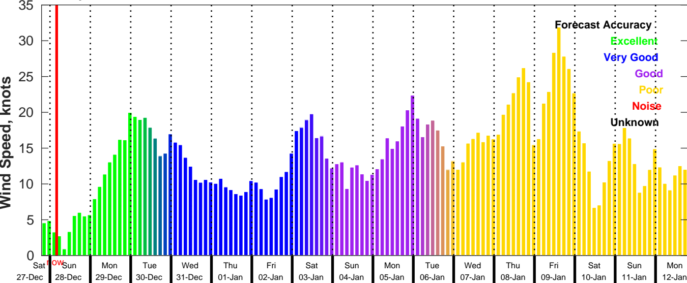
GFS Wind Speed Forecast for NDBC 42036 from 27-Dec-2025 19:00:00 to 12-Jan-2026 19:00:00
