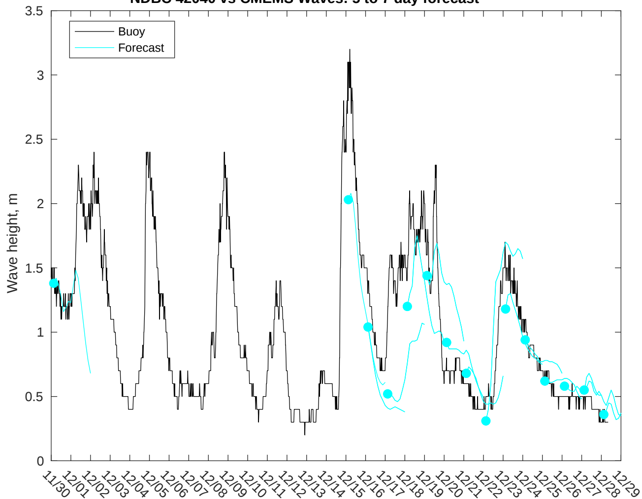
NDBC 42040 vs CMEMS Waves: 5 to 7 day forecast
