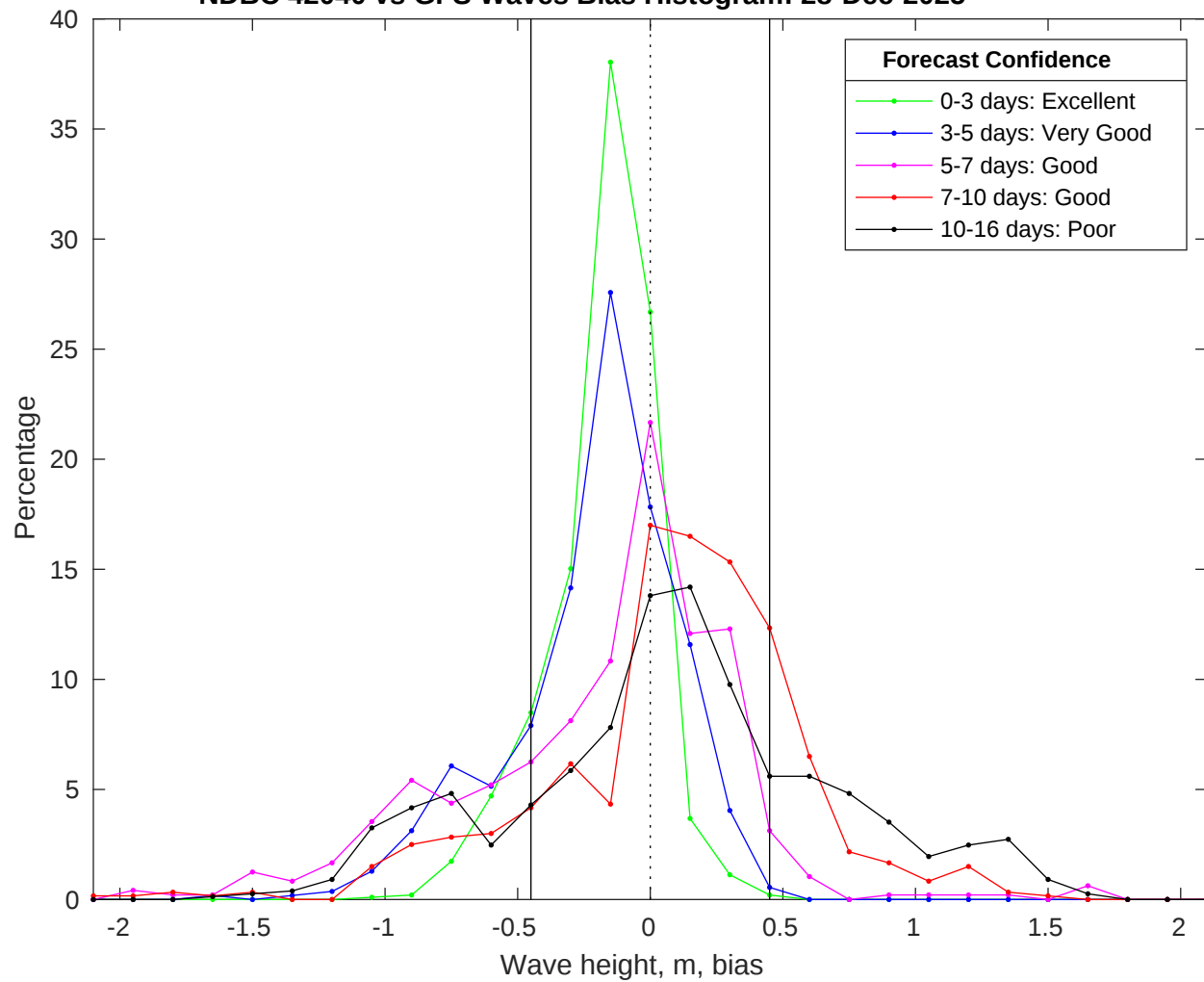
NDBC 42040 vs GFS Waves Bias Histogram: 28-Dec-2025
