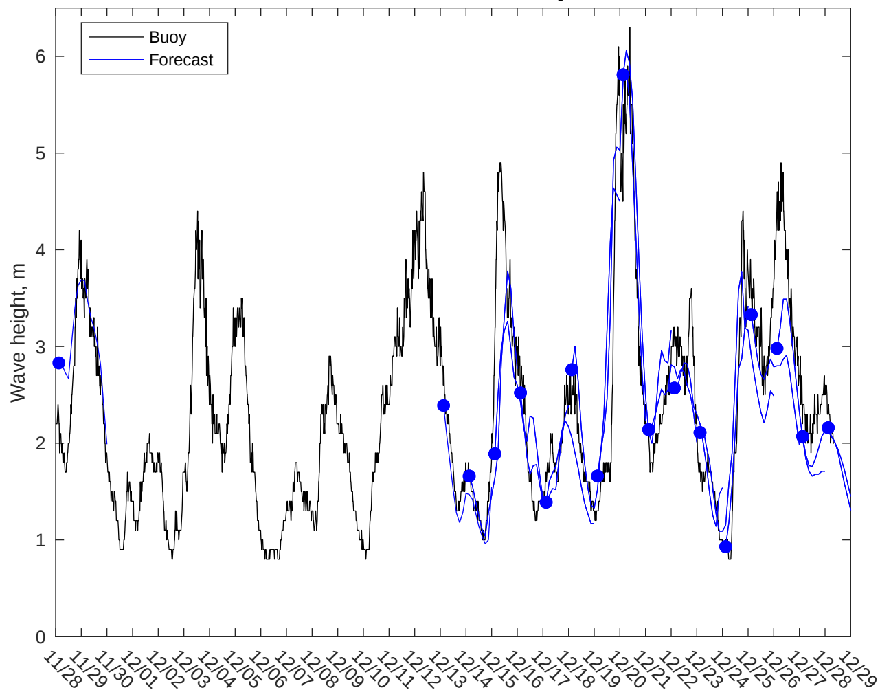
NDBC 44008 vs CMEMS Waves: 3 to 5 day forecast
