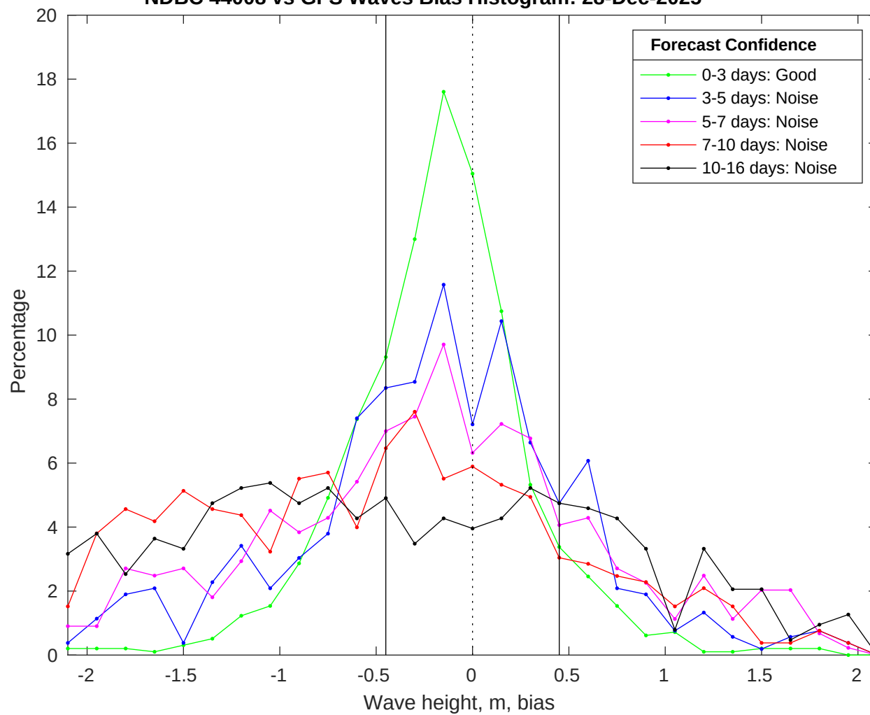
NDBC 44008 vs GFS Waves Bias Histogram: 28-Dec-2025
