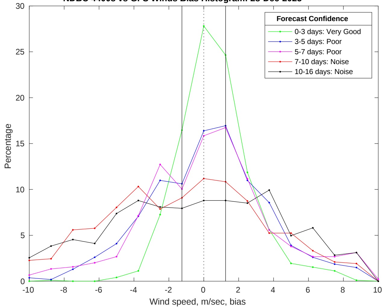
NDBC 44008 vs GFS Winds Bias Histogram: 28-Dec-2025
