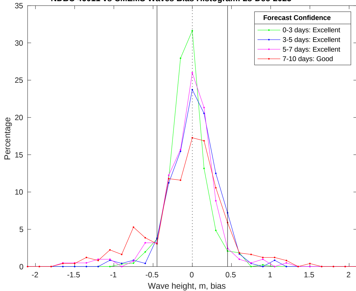
NDBC 46011 vs CMEMS Waves Bias Histogram: 28-Dec-2025
