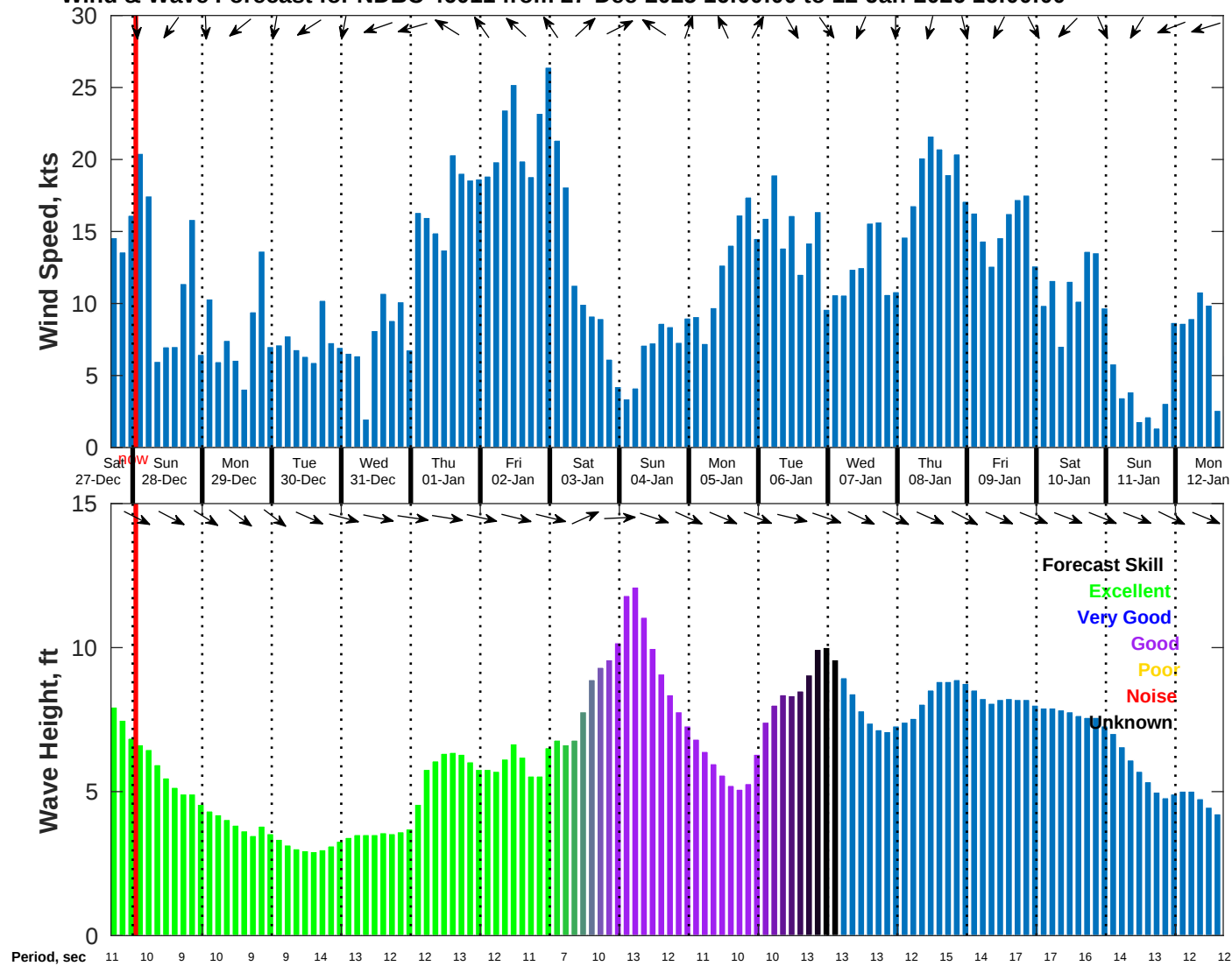
Wind & Wave Forecast for NDBC 46011 from 27-Dec-2025 16:00:00 to 12-Jan-2026 16:00:00
