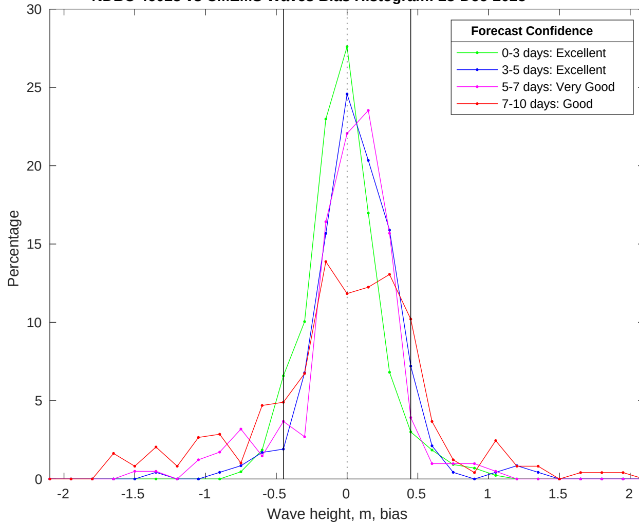
NDBC 46028 vs CMEMS Waves Bias Histogram: 28-Dec-2025
