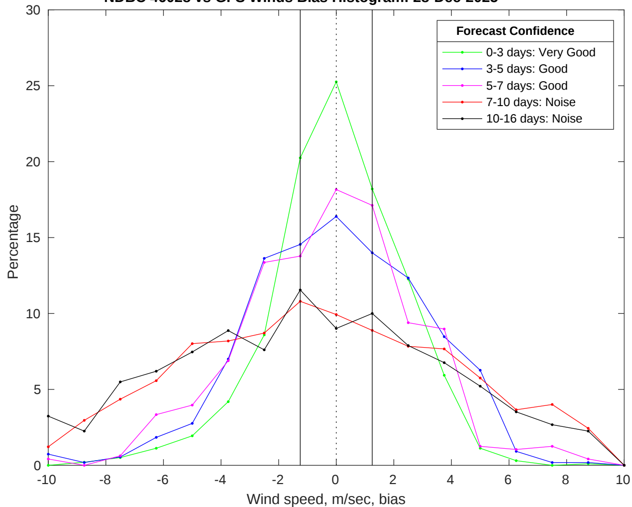
NDBC 46028 vs GFS Winds Bias Histogram: 28-Dec-2025
