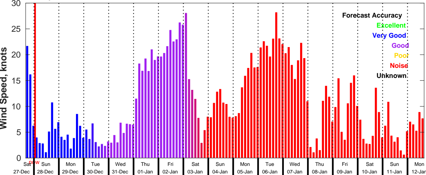
GFS Wind Speed Forecast for NDBC 46028 from 27-Dec-2025 16:00:00 to 12-Jan-2026 16:00:00
