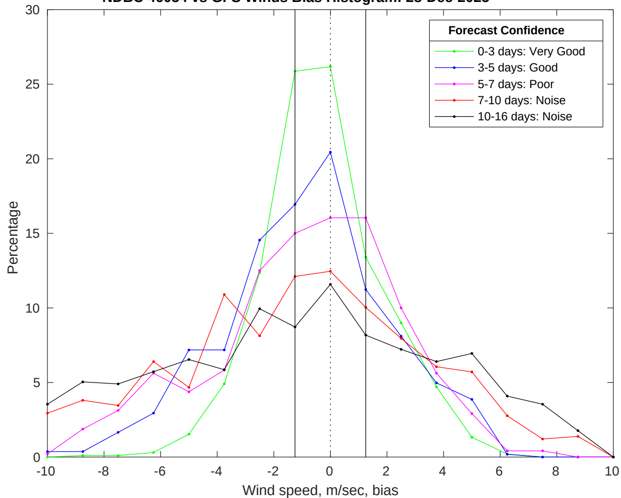
NDBC 46054 vs GFS Winds Bias Histogram: 28-Dec-2025
