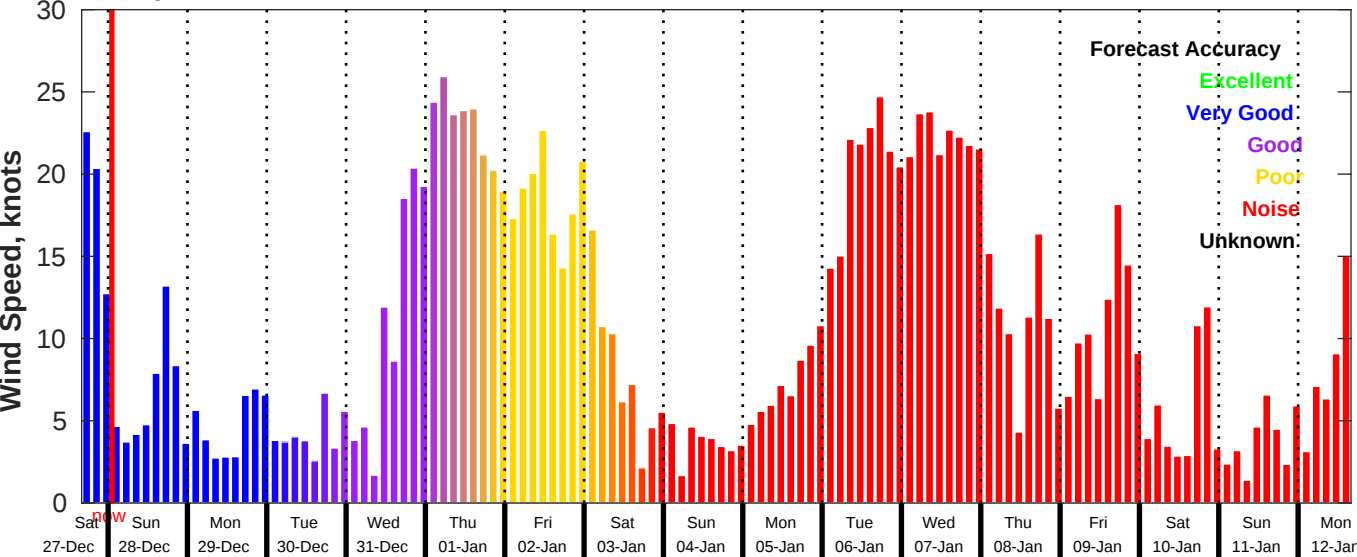
GFS Wind Speed Forecast for NDBC 46054 from 27-Dec-2025 16:00:00 to 12-Jan-2026 16:00:00
