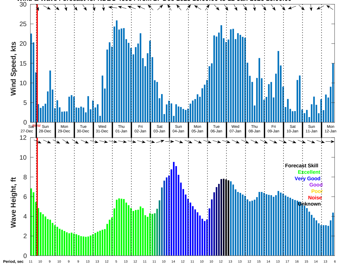
Wind & Wave Forecast for NDBC 46054 from 27-Dec-2025 16:00:00 to 12-Jan-2026 16:00:00
