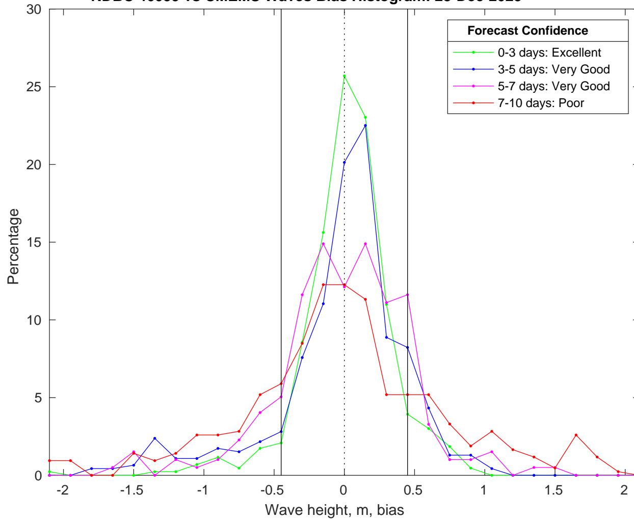
NDBC 46059 vs CMEMS Waves Bias Histogram: 28-Dec-2025
