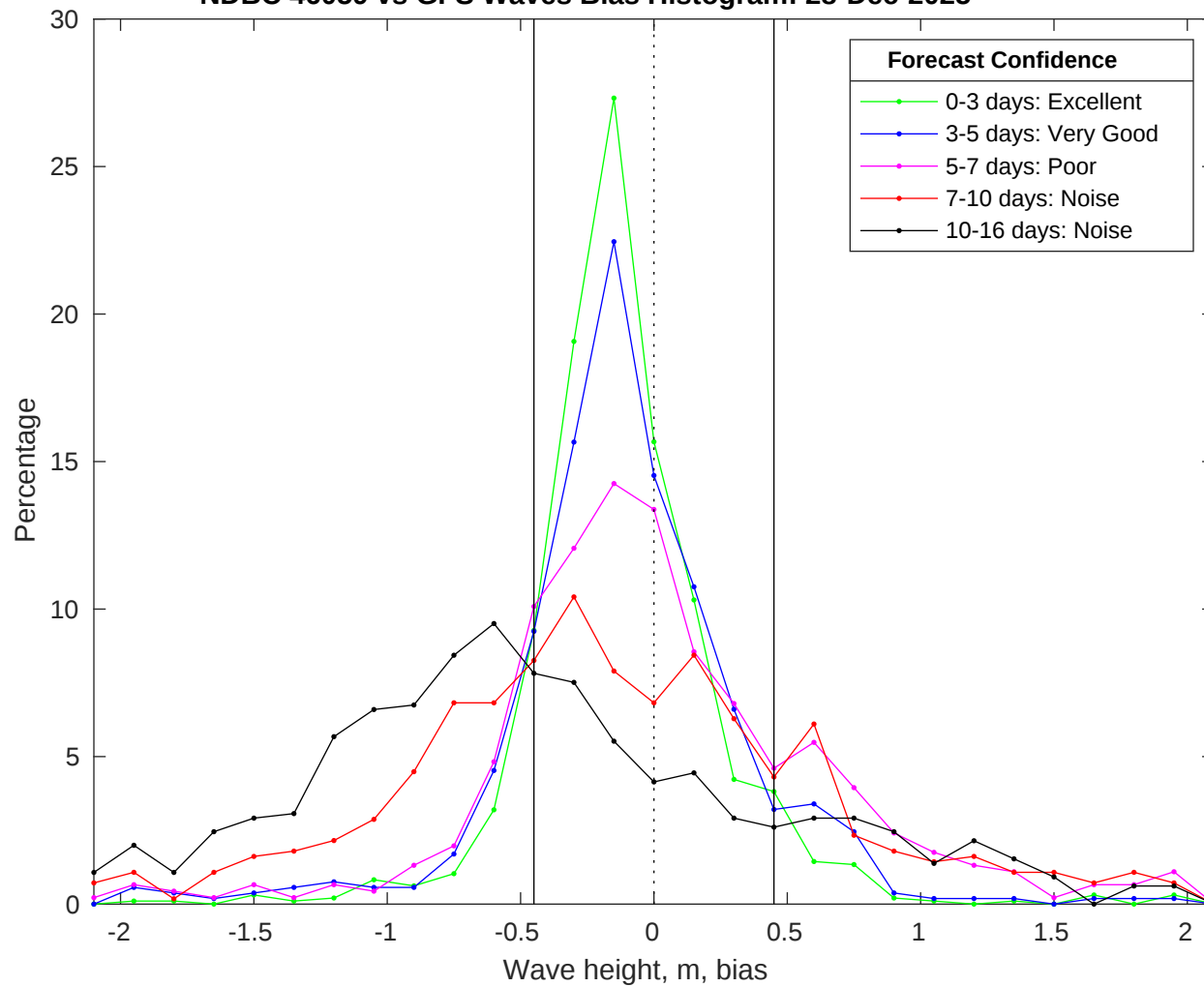
NDBC 46059 vs GFS Waves Bias Histogram: 28-Dec-2025
