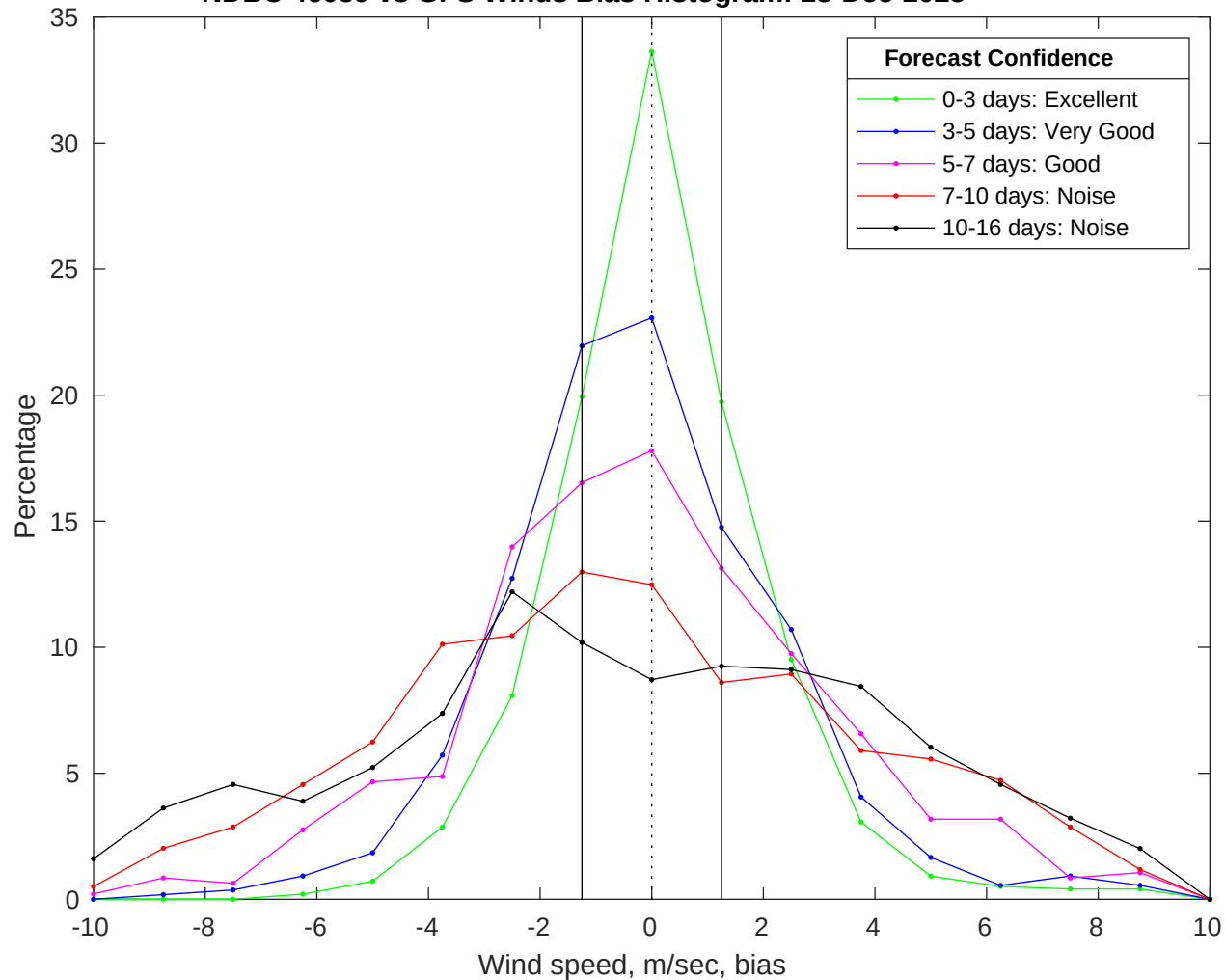
NDBC 46059 vs GFS Winds Bias Histogram: 28-Dec-2025
