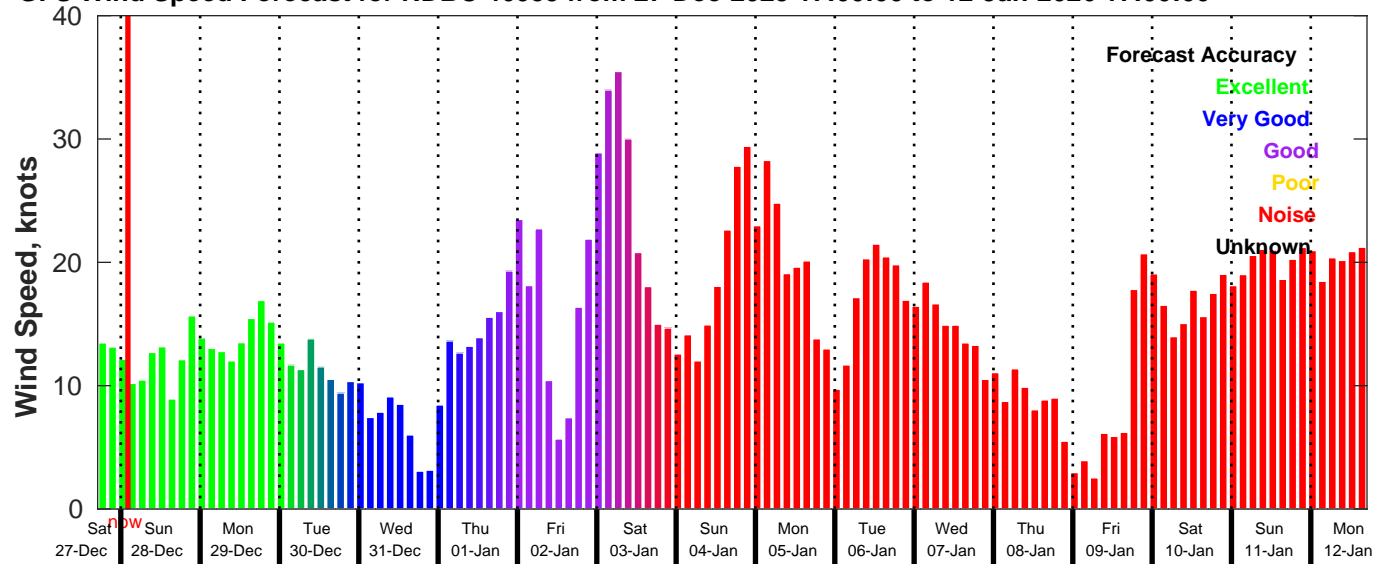
GFS Wind Speed Forecast for NDBC 46059 from 27-Dec-2025 17:00:00 to 12-Jan-2026 17:00:00
