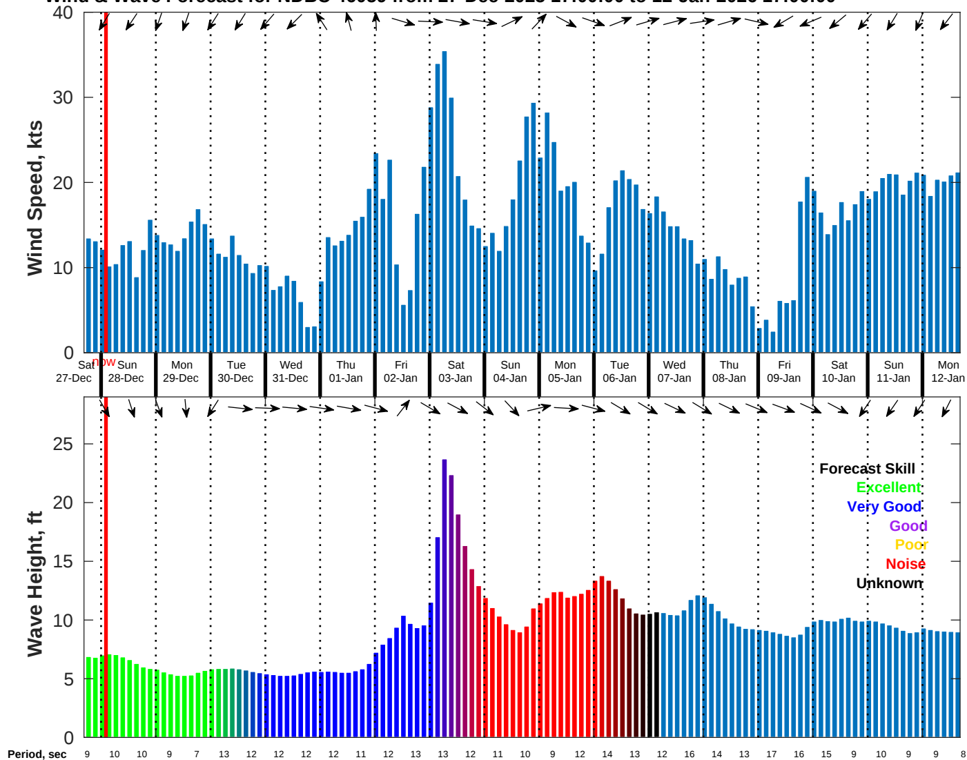
Wind & Wave Forecast for NDBC 46059 from 27-Dec-2025 17:00:00 to 12-Jan-2026 17:00:00
