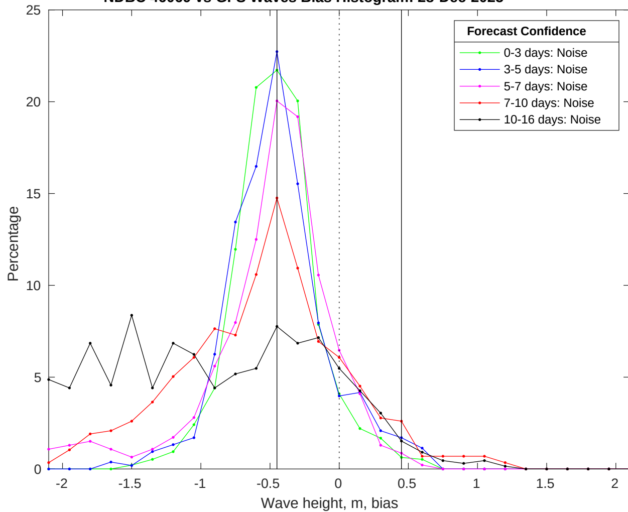
NDBC 46069 vs GFS Waves Bias Histogram: 28-Dec-2025
