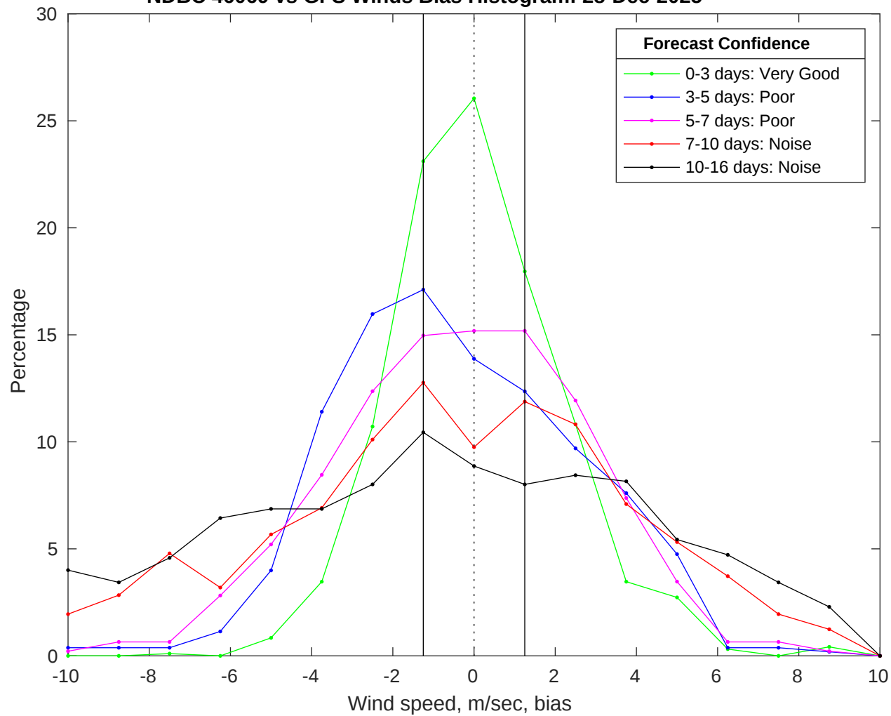
NDBC 46069 vs GFS Winds Bias Histogram: 28-Dec-2025
