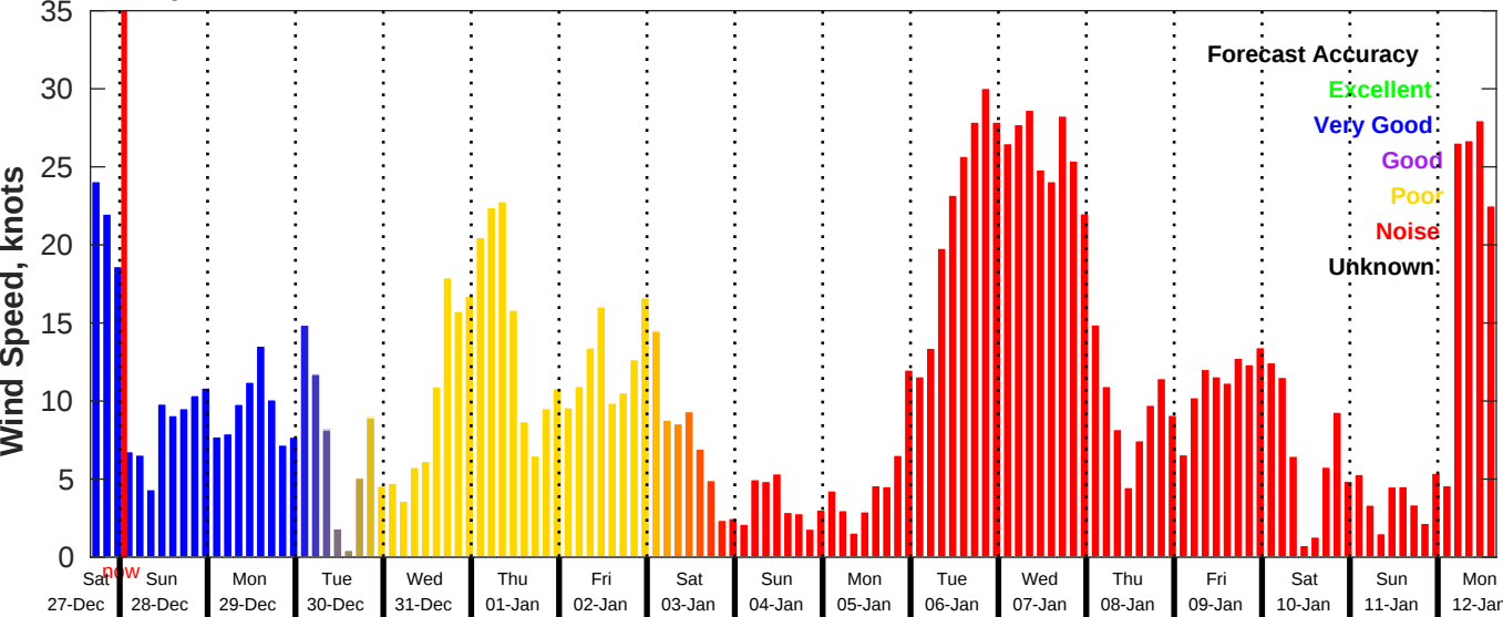
GFS Wind Speed Forecast for NDBC 46069 from 27-Dec-2025 16:00:00 to 12-Jan-2026 16:00:00
