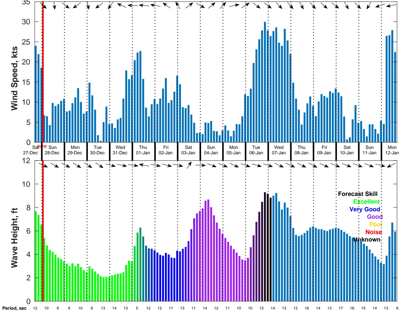
Wind & Wave Forecast for NDBC 46069 from 27-Dec-2025 16:00:00 to 12-Jan-2026 16:00:00
