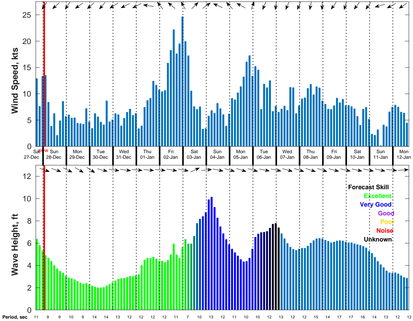
Wind & Wave Forecast for NDBC 46215 from 27-Dec-2025 16:00:00 to 12-Jan-2026 16:00:00
