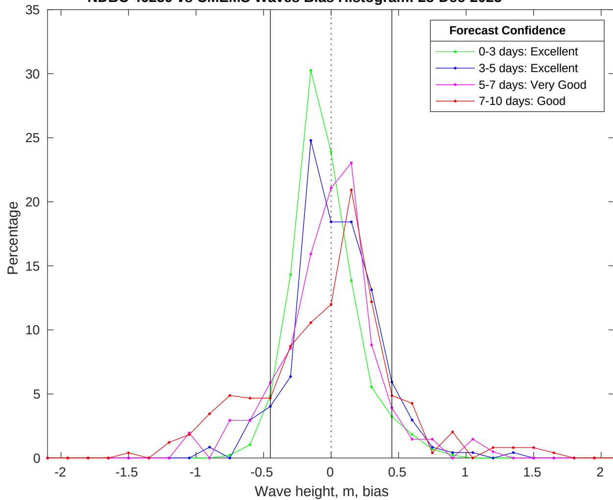
NDBC 46259 vs CMEMS Waves Bias Histogram: 28-Dec-2025
