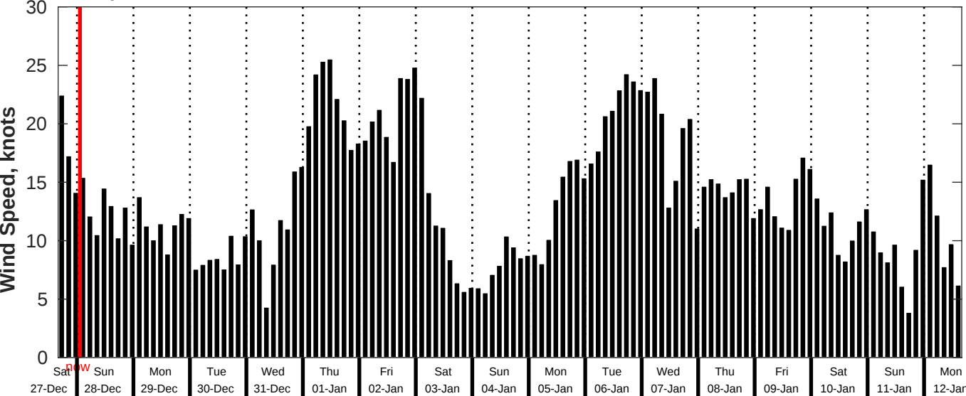
GFS Wind Speed Forecast for NDBC 46259 from 27-Dec-2025 16:00:00 to 12-Jan-2026 16:00:00
