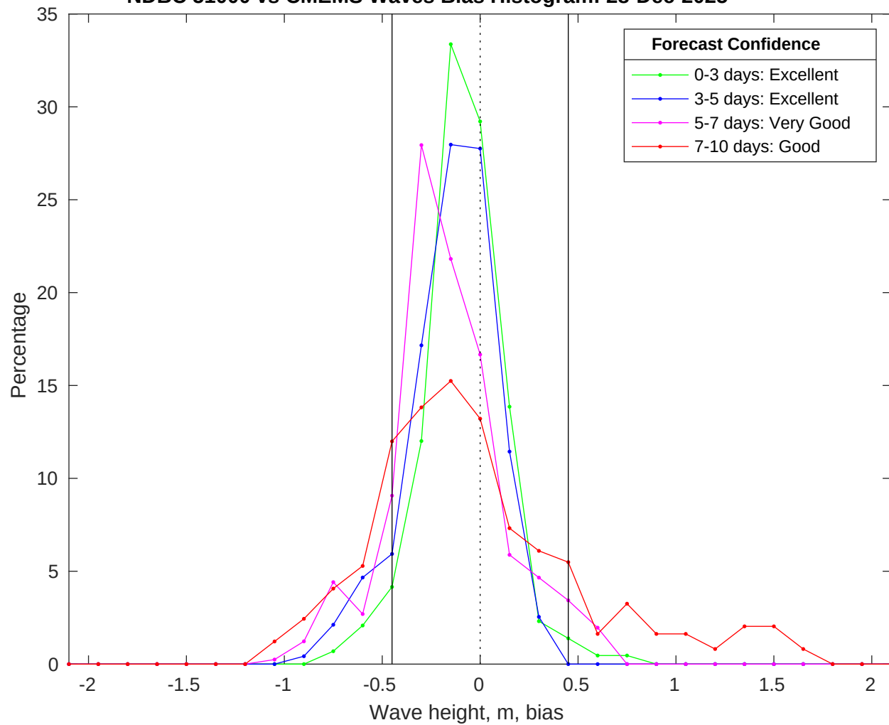
NDBC 51000 vs CMEMS Waves Bias Histogram: 28-Dec-2025
