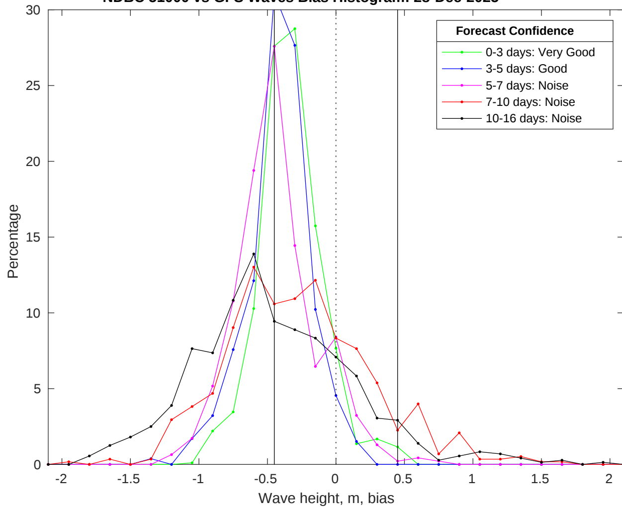
NDBC 51000 vs GFS Waves Bias Histogram: 28-Dec-2025
