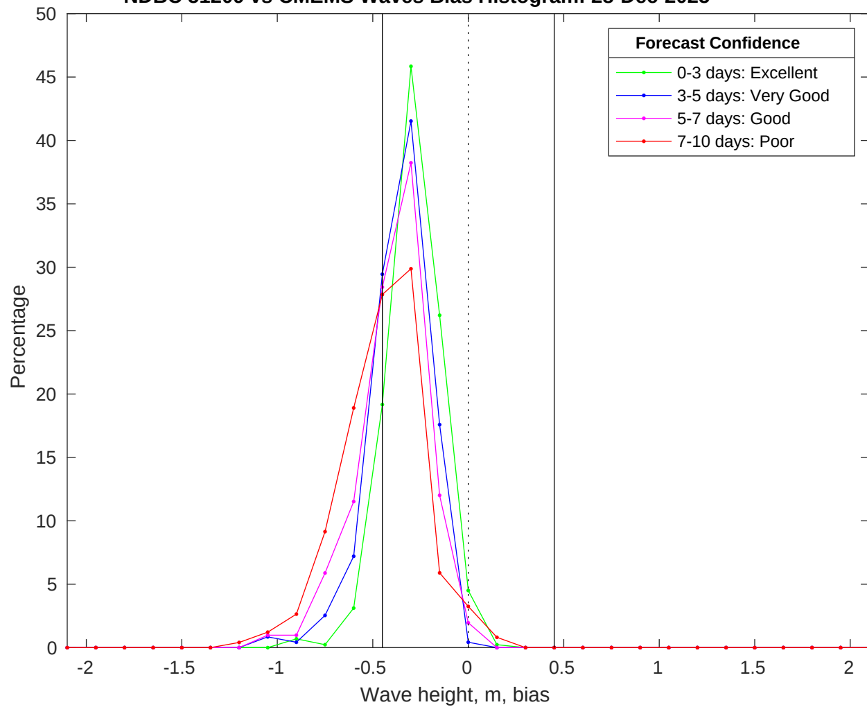
NDBC 51209 vs CMEMS Waves Bias Histogram: 28-Dec-2025
