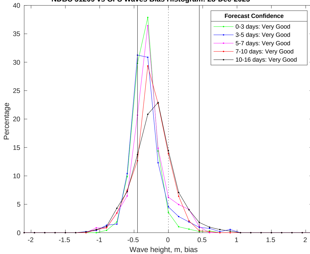
NDBC 51209 vs GFS Waves Bias Histogram: 28-Dec-2025
