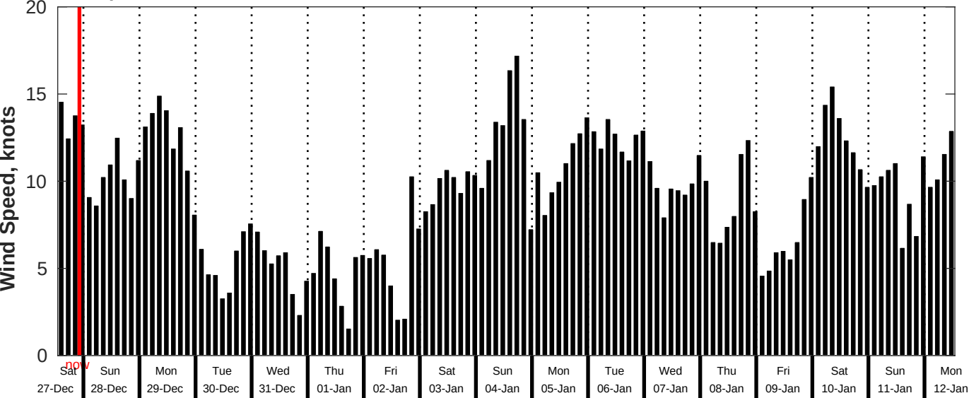
GFS Wind Speed Forecast for NDBC 51209 from 27-Dec-2025 13:00:00 to 12-Jan-2026 13:00:00
