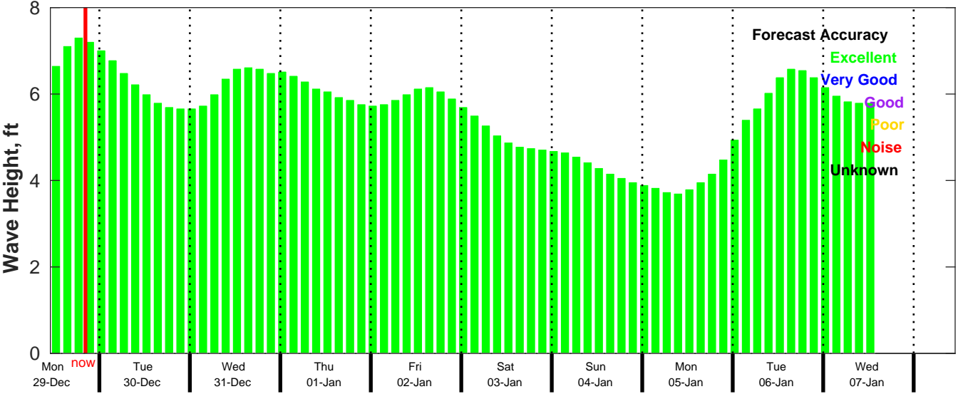
CMEMS Wave Forecast for NDBC 52211 from 28-Dec-2025 11:00:00 to 07-Jan-2026 11:00:00
