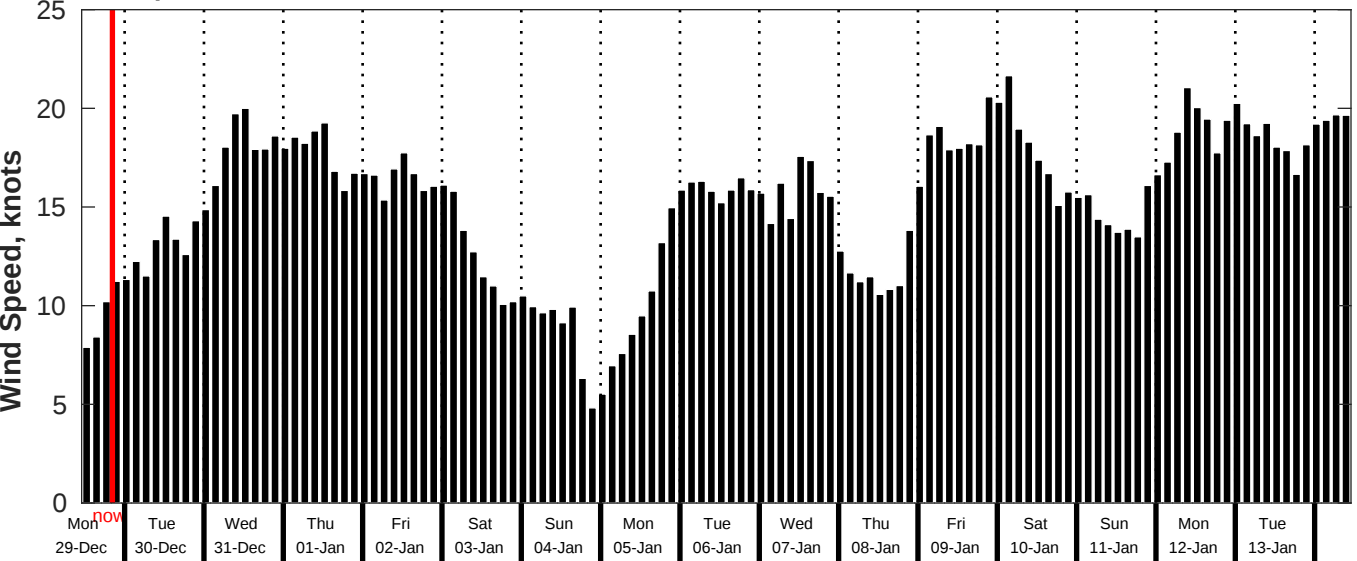
GFS Wind Speed Forecast for NDBC 52211 from 28-Dec-2025 11:00:00 to 13-Jan-2026 11:00:00
