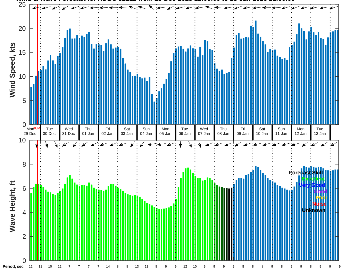
Wind & Wave Forecast for NDBC 52211 from 28-Dec-2025 11:00:00 to 13-Jan-2026 11:00:00
