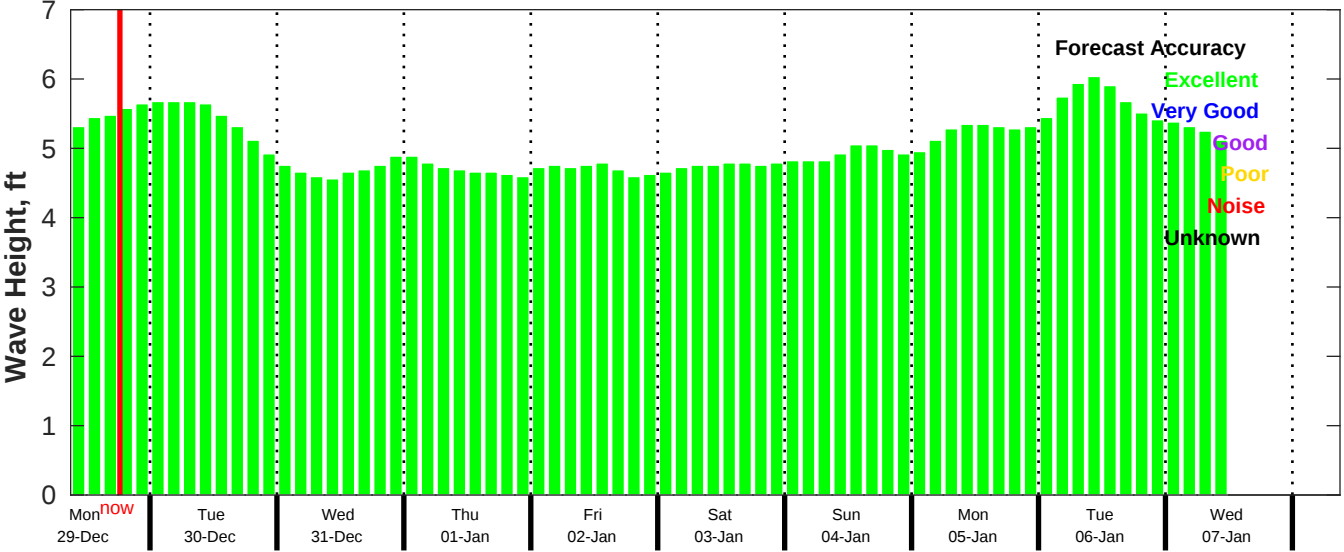
CMEMS Wave Forecast for NDBC 52212 from 28-Dec-2025 09:00:00 to 07-Jan-2026 09:00:00
