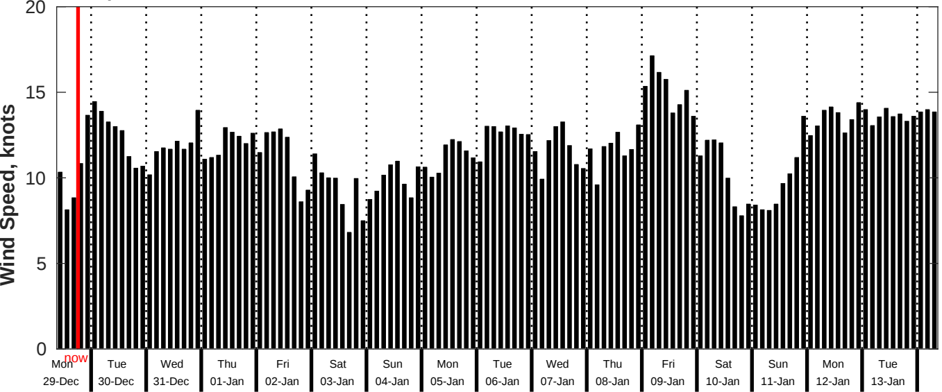
GFS Wind Speed Forecast for NDBC 52212 from 28-Dec-2025 09:00:00 to 13-Jan-2026 09:00:00
