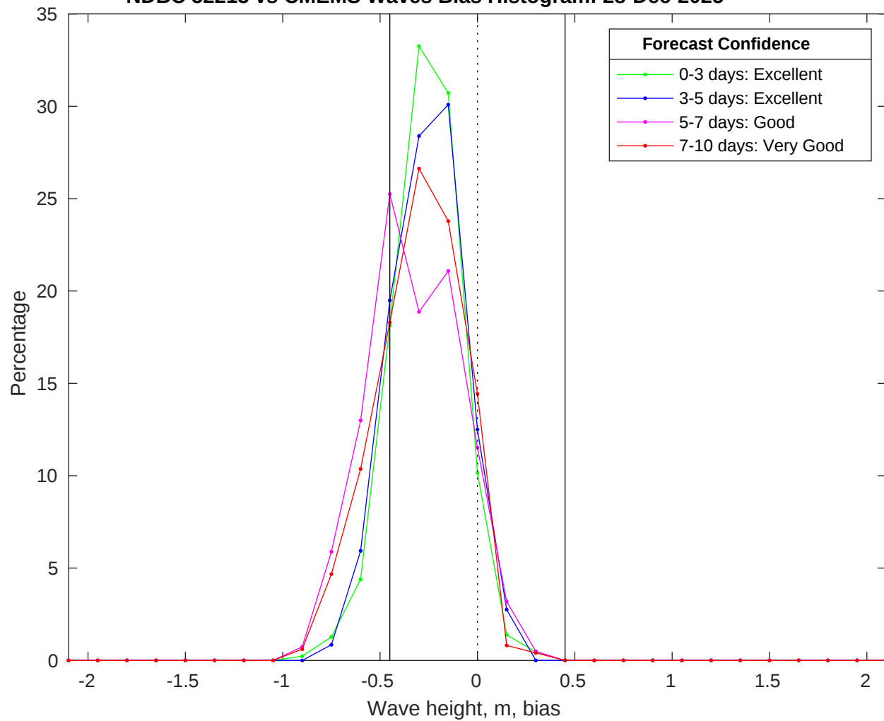
NDBC 52213 vs CMEMS Waves Bias Histogram: 28-Dec-2025
