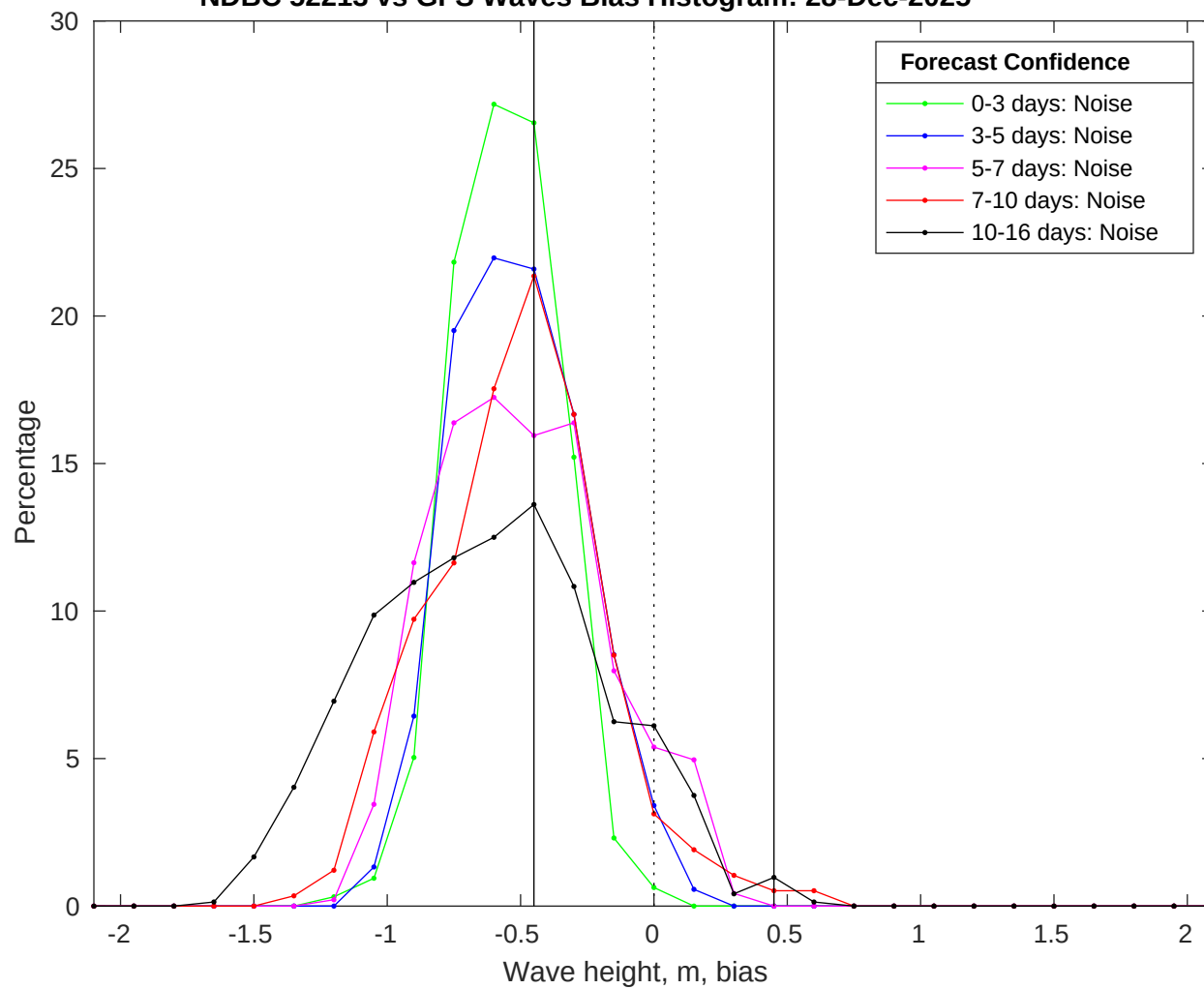
NDBC 52213 vs GFS Waves Bias Histogram: 28-Dec-2025
