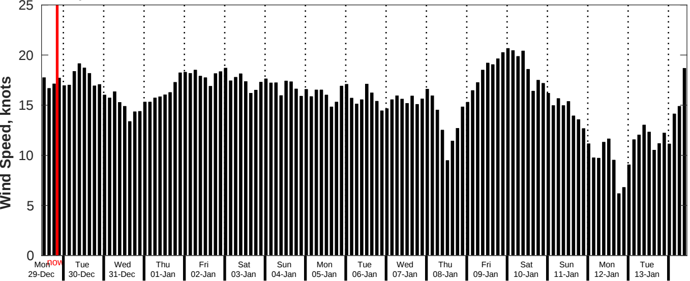
GFS Wind Speed Forecast for NDBC 52213 from 28-Dec-2025 11:00:00 to 13-Jan-2026 11:00:00
