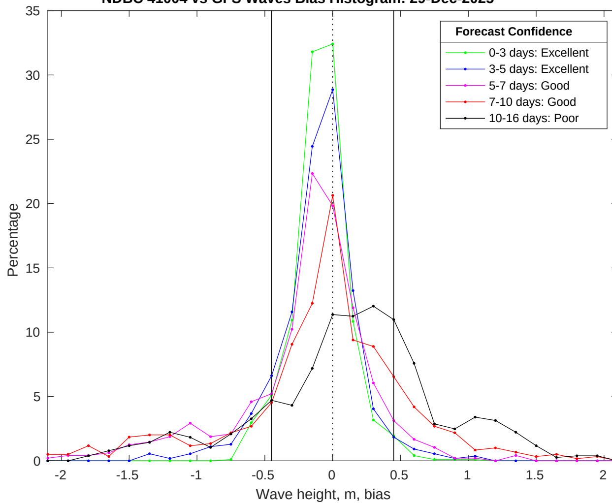
NDBC 41004 vs GFS Waves Bias Histogram: 29-Dec-2025
