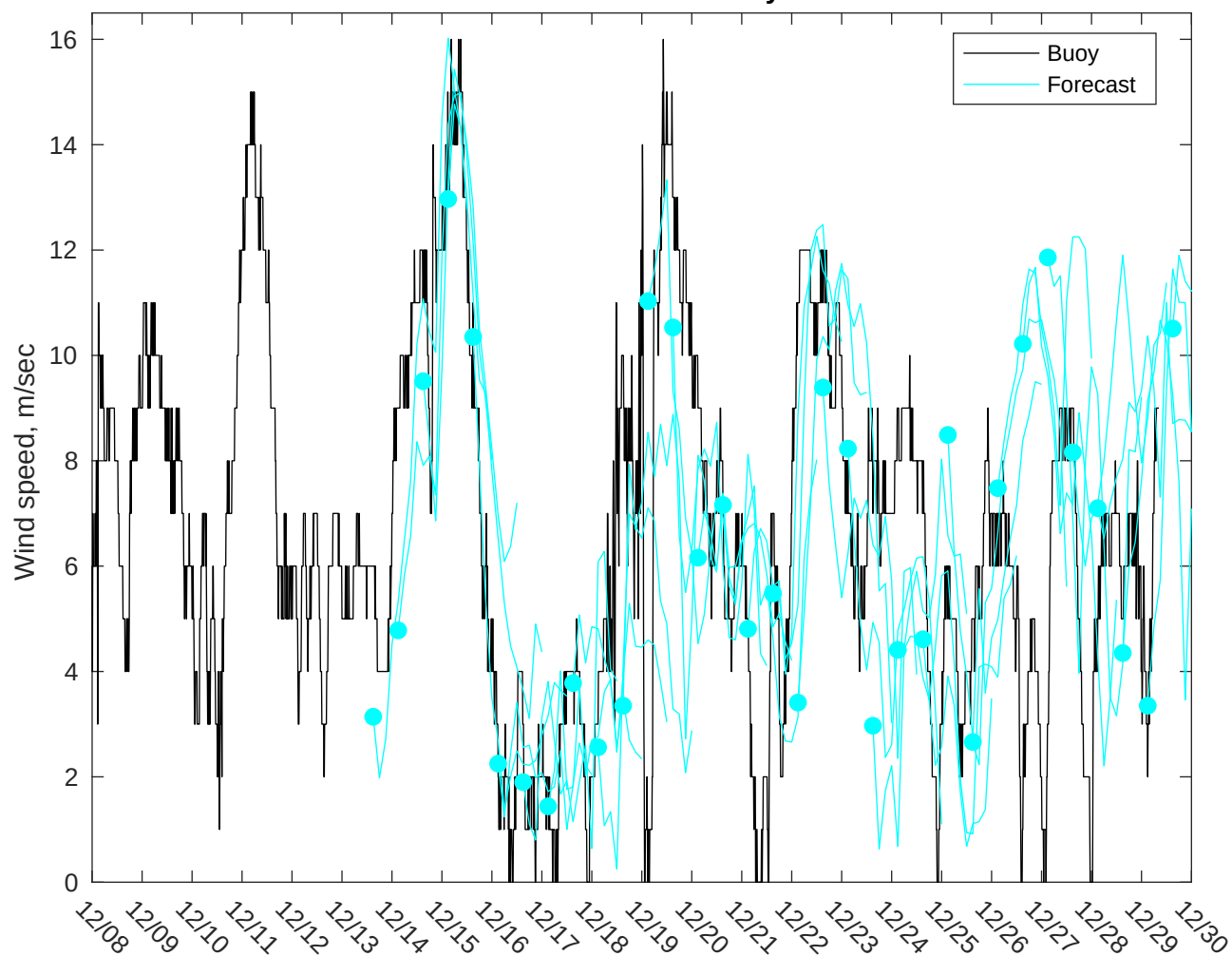
NDBC 41004 vs GFS Winds: 5 to 7 day forecast
