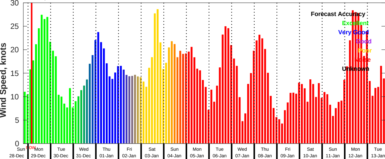
GFS Wind Speed Forecast for NDBC 41004 from 28-Dec-2025 19:00:00 to 13-Jan-2026 19:00:00
