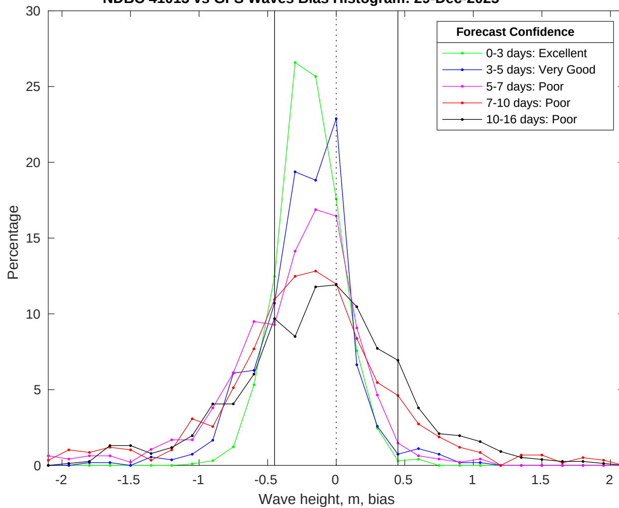
NDBC 41013 vs GFS Waves Bias Histogram: 29-Dec-2025
